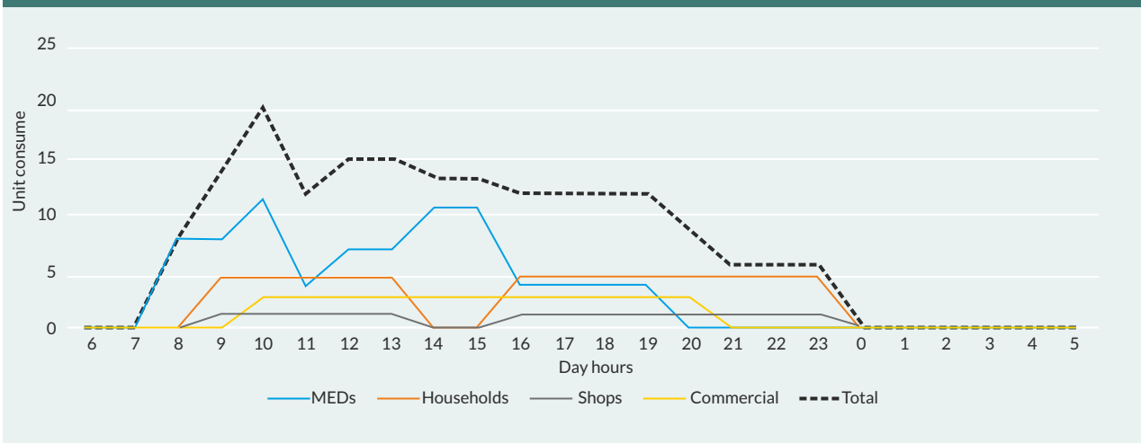
Figure 2.2: A typical load curve of a mini-grid site
